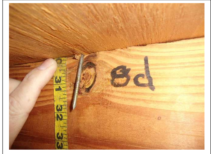
ROOF DECK ATTACHEMNT – 8d common nails added in 2006
